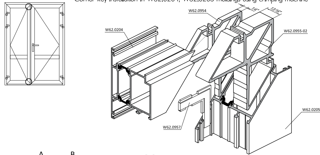
Corner key installation in W62.0204, W62.0205 moldings using crimping machine
