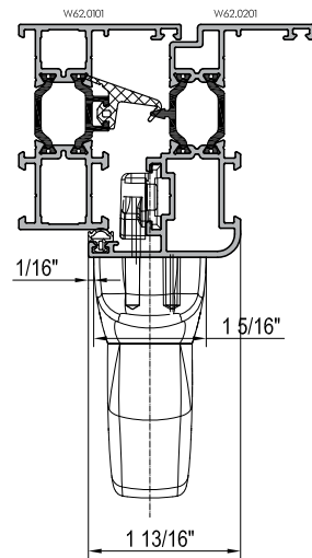
Window handle NEFER 0760B
