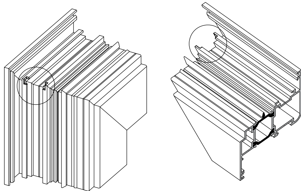
Notches for hardware
