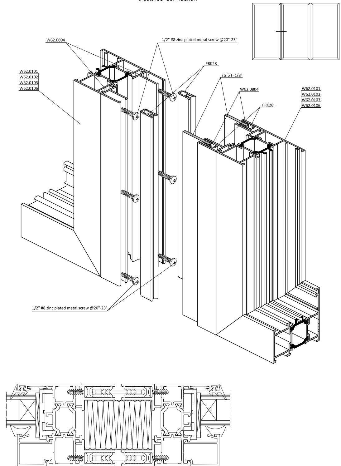
Insulated connection
