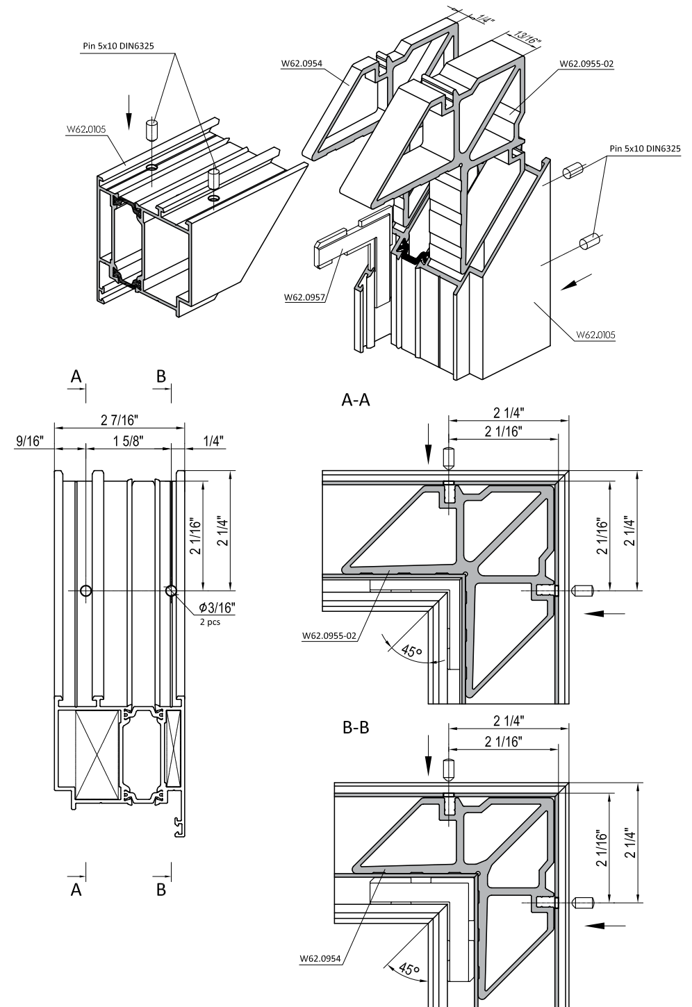
Corner key installation in W62.0105 moldings using pins. Variant 2
