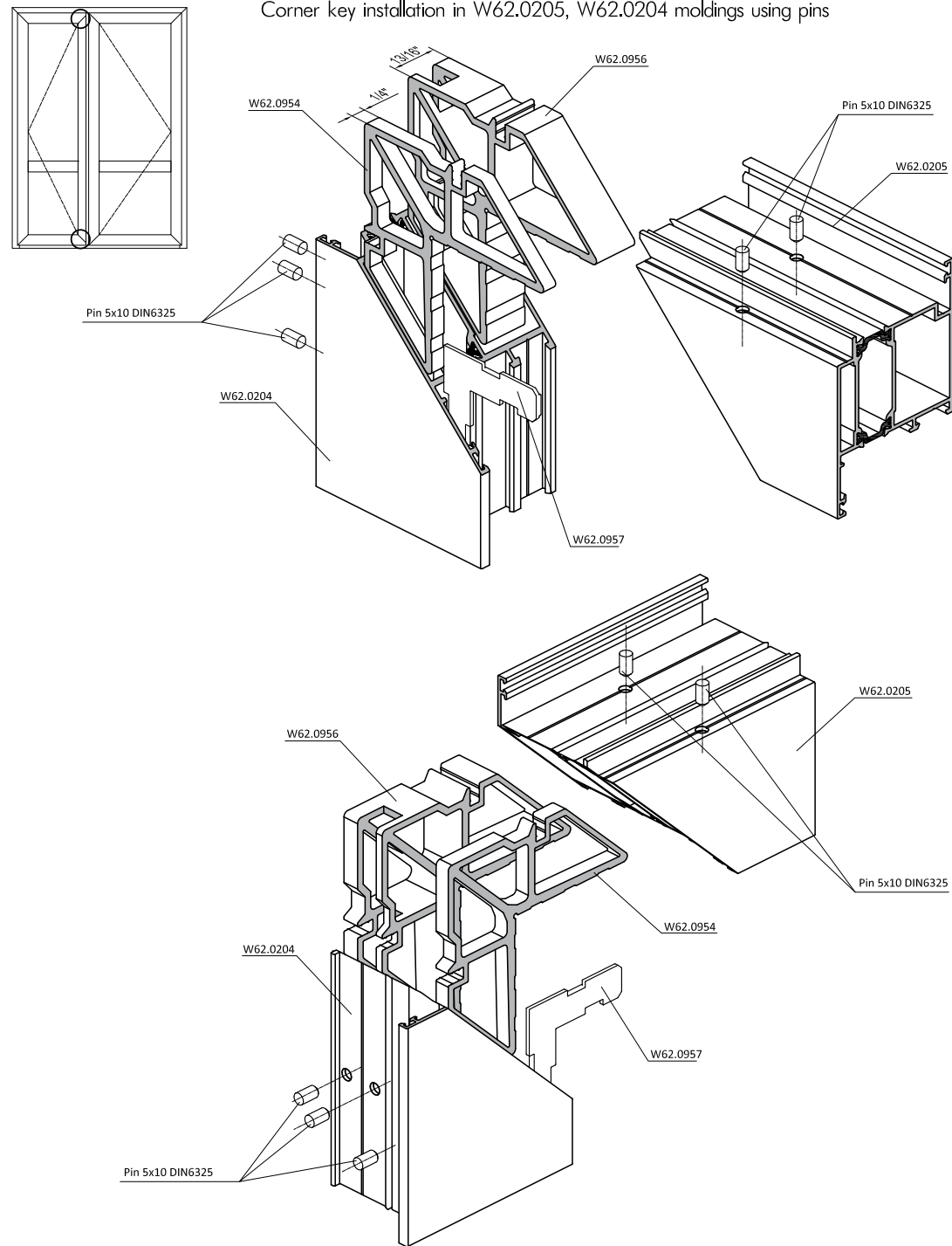
Corner key installation in W62.0205, W62.0204 moldings using pins
