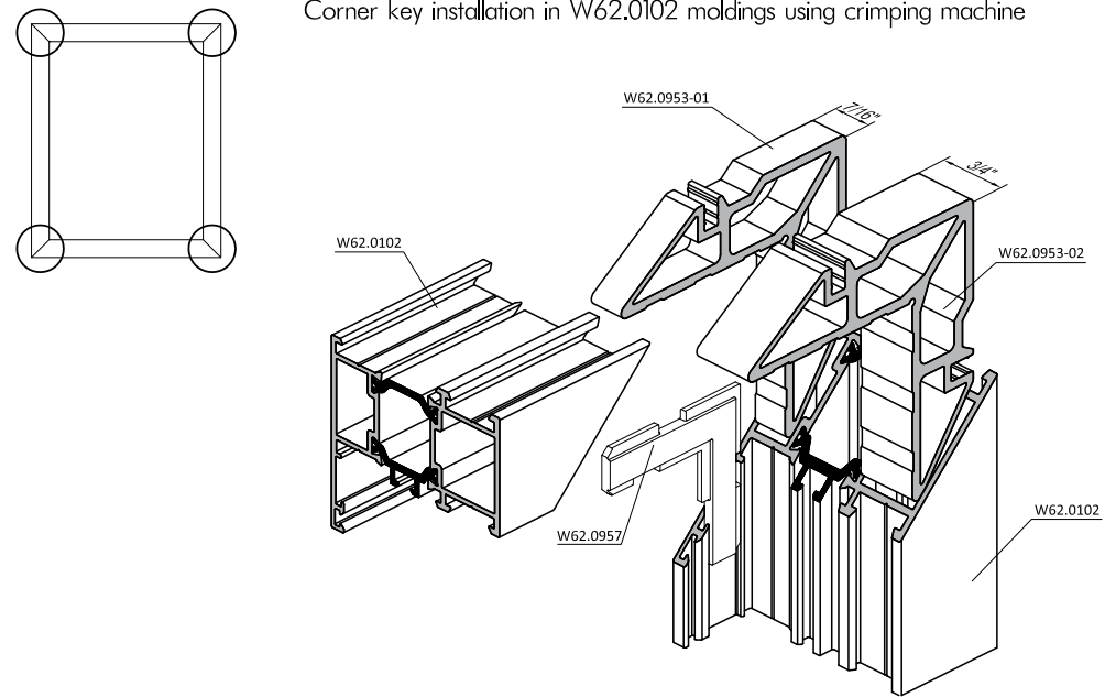
Corner key installation in W62.0102 moldings using crimping machine
