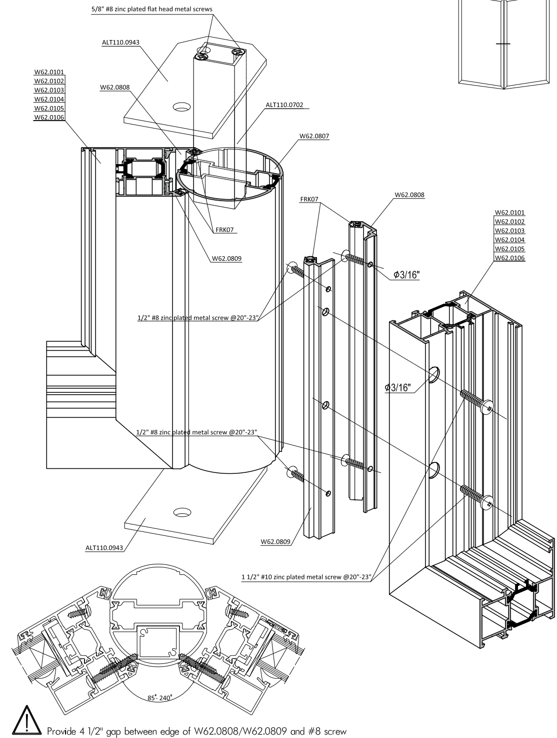
85° - 240° corner assembly
