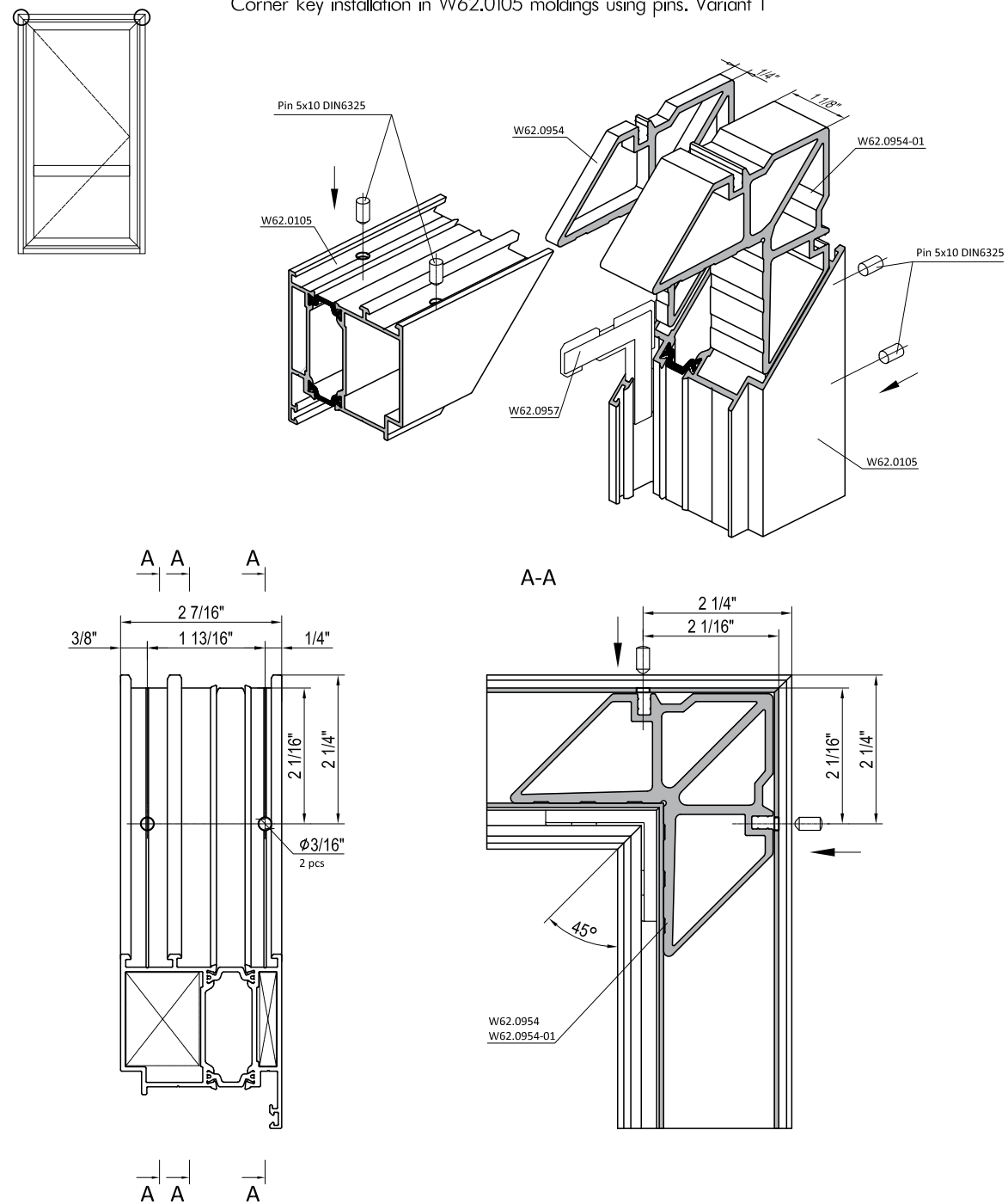
Corner key installation in W62.0105 moldings using pins. Variant 1
